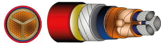
Three Core Belted Paper
