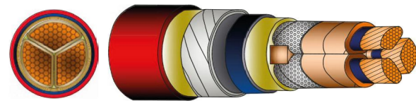
Three Core Screened Paper
