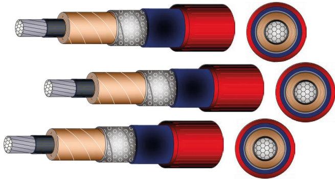
Single Core Paper Lead
