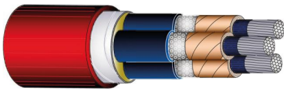
Three Core Paper Single Lead
